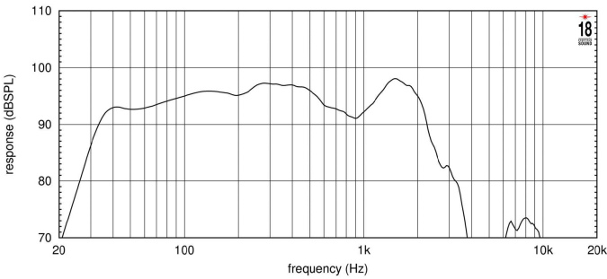
FREQUENCY RESPONSE CURVE OF 18NLW9601 MADE ON 180 LIT. ENCLOSURE TUNED AT 35HZ IN FREE FIELD (4PI) ENVIRONMENT. ENCLOSURE CLOSES THE REAR OF THE DRIVER. THE THIN LINE REPRESENTS 45 DEG. OFF AXIS FREQUENCY RESPONSE
