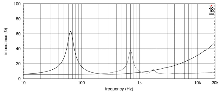
FREQUENCY RESPONSE MADE IN 25 LT. ENCLOSURE TUNED AT 65 Hz IN FREE FIELD (4n) ENVIRONMENT. ENCLOSURE CLOSES THE REAR OF THE DRIVER, THE THIN LINE REPRESENTS HIGH FREQUENCY FREE AIR IMPEDANCE MAGNITUDE CURVE
