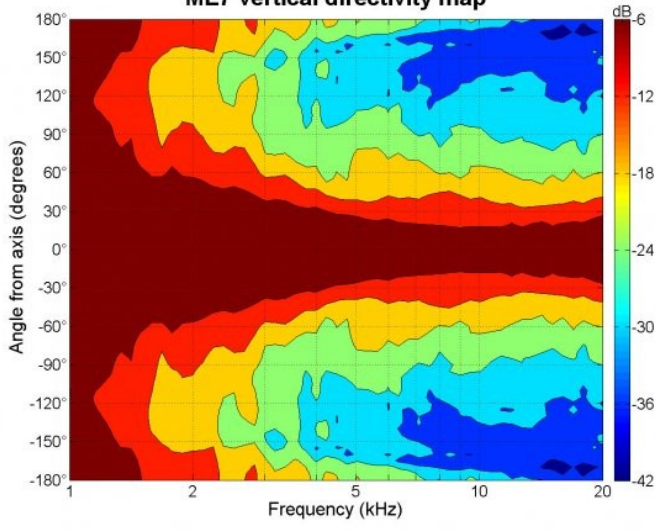
ME7 vertical directivity map
