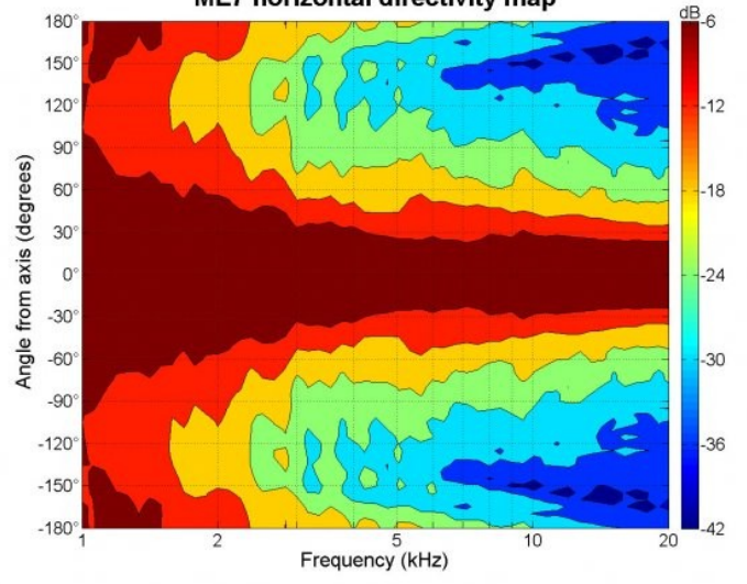
ME7 horizontal directivity map
