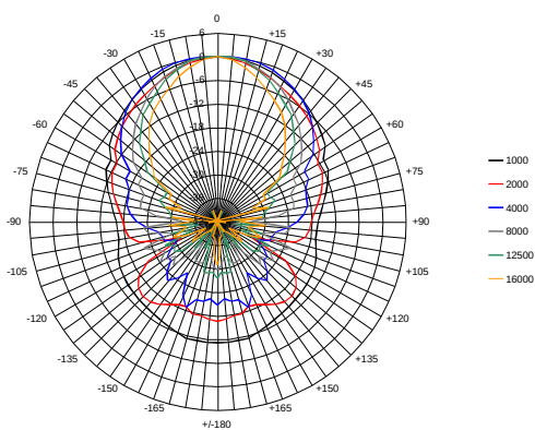
Q07015A Horizontal Polar Pattern
