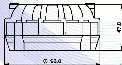
Mounting holes: 2 holes M6 on Ø70mm
